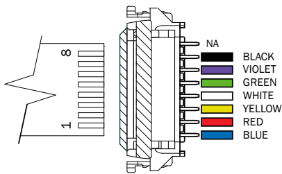
Socket Wiring (Cap unused wires)
